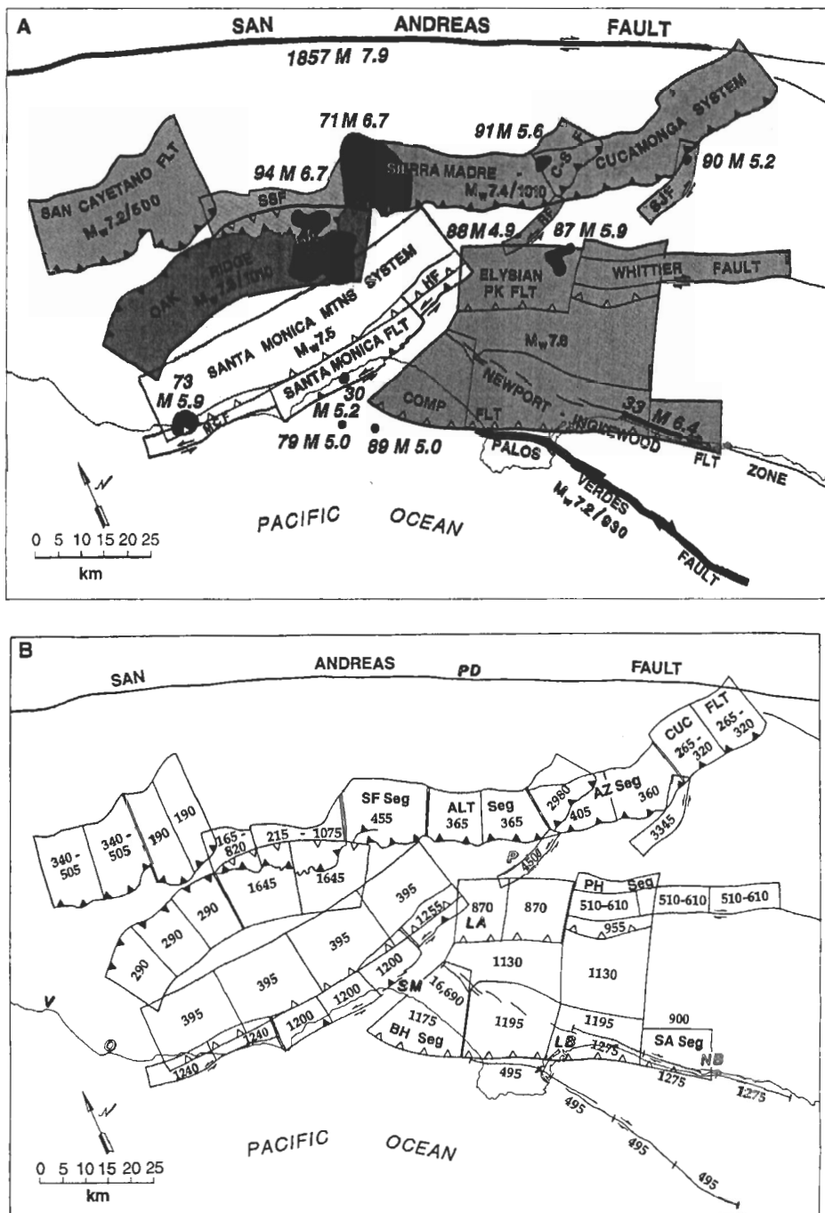
Fig. 1. (A) Historical earthquake ruptures and proposed large earthquake sources within the greater Los Angeles metropolitan area. Black areas denote surface projections of rupture planes of selected moderate historic earthquakes (6, 35–40, 65–67). Date and magnitude ( M_w ) of each earthquake are also shown. Historic ruptures on vertical strike-slip faults (1857 and 1933 earthquakes) are shown as heavy black lines. Polygons represent map projections of nonvertical fault planes. Thin lines denote near-vertical faults. Intermediate-width lines outline major fault systems that we consider could cause large earthquakes ( M_w 7.2 to 7.6). Solid barsbs denote thrust faults that break the surface; barbs point downdip. Open barbs represent the upper edge of blind thrust fault ramps; barbs point downdip. Predominantly strike-slip faults are shown by double arrows along the surficial trace of each fault. Maximum credible earthquakes and their average recurrence intervals are shown for each fault system (for example, M_w 7.4/1010 on the Sierra Madre system indicates a recurrence interval of approximately 1010 years for a M_w 7.4 earthquake rupturing the entire system). Comp FLT, Compton fault; C-SF, Clamshell-Sawpit fault; HF, Hollywood fault; MCF, Malibu Coast fault; RF, Raymond fault; SJF, San José fault; SSF, Santa Susana fault. (B) Map showing the 51 potential, moderate ( M_w 6.5 to 6.8; average M_w 6.7) earthquake sources within the metropolitan region that we used in our moderate-earthquake scenario. The number within each earthquake source area denotes the approximate average recurrence interval (in years) for a moderate earthquake from each source region. In this scenario, for example, the source of the Northridge earthquake produces a M_w 6.7 event every 1645 years. Double lines denote geologically reasonable segment boundaries. ALT Seg, Altadena segment; AZ Seg, Azusa segment; BH Seg, Baldwin Hills segment; CUC FLT, Cucamonga fault; LA, downtown Los Angeles; LB, Long Beach; NB, Newport Beach; O, Oxnard; P, Pasadena; PD, Palmdale; PH Seg, Puente Hills segment; SA Seg, Santa Ana segment; SF Seg, San Fernando segment; SM, Santa Monica; V, Ventura.
